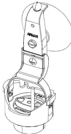
Figure 12. P48W or TM150M: Portable Bracket (P48W shown) Airmar Part No. 33-076-01 Copyright © 2008 - 2012 Airmar Technology Corp.
